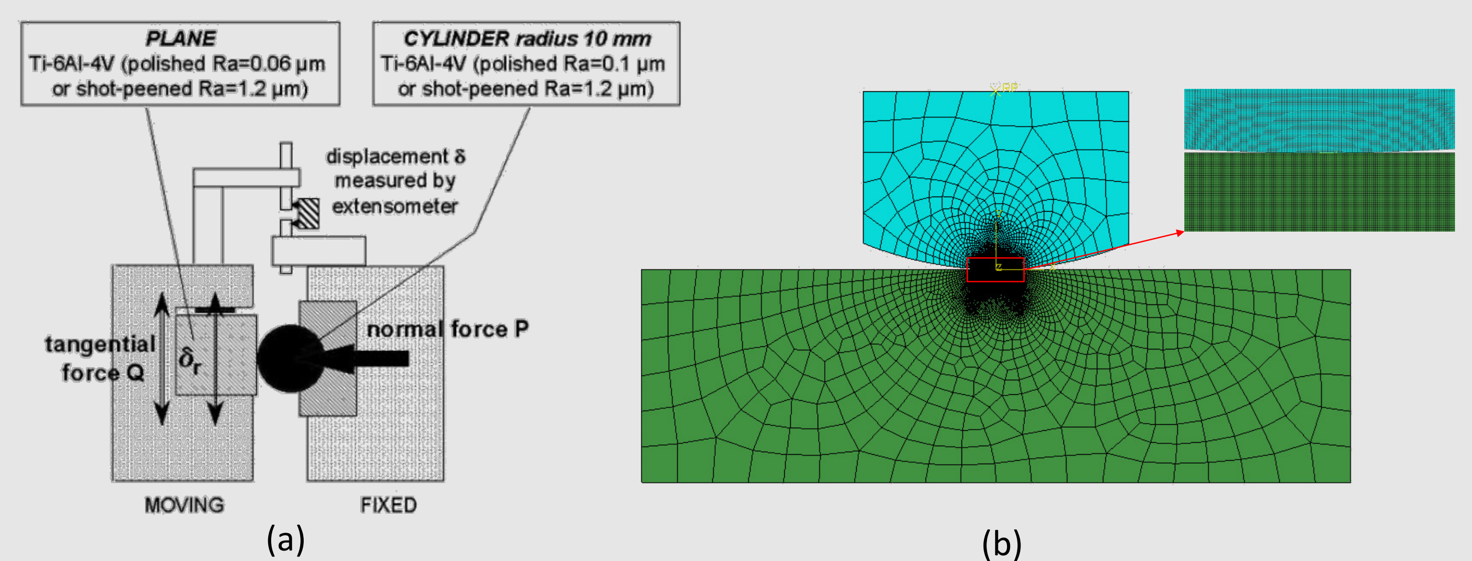
Fig. 2. The experimental setup (a) and the finite element model (b) for fretting wear.
