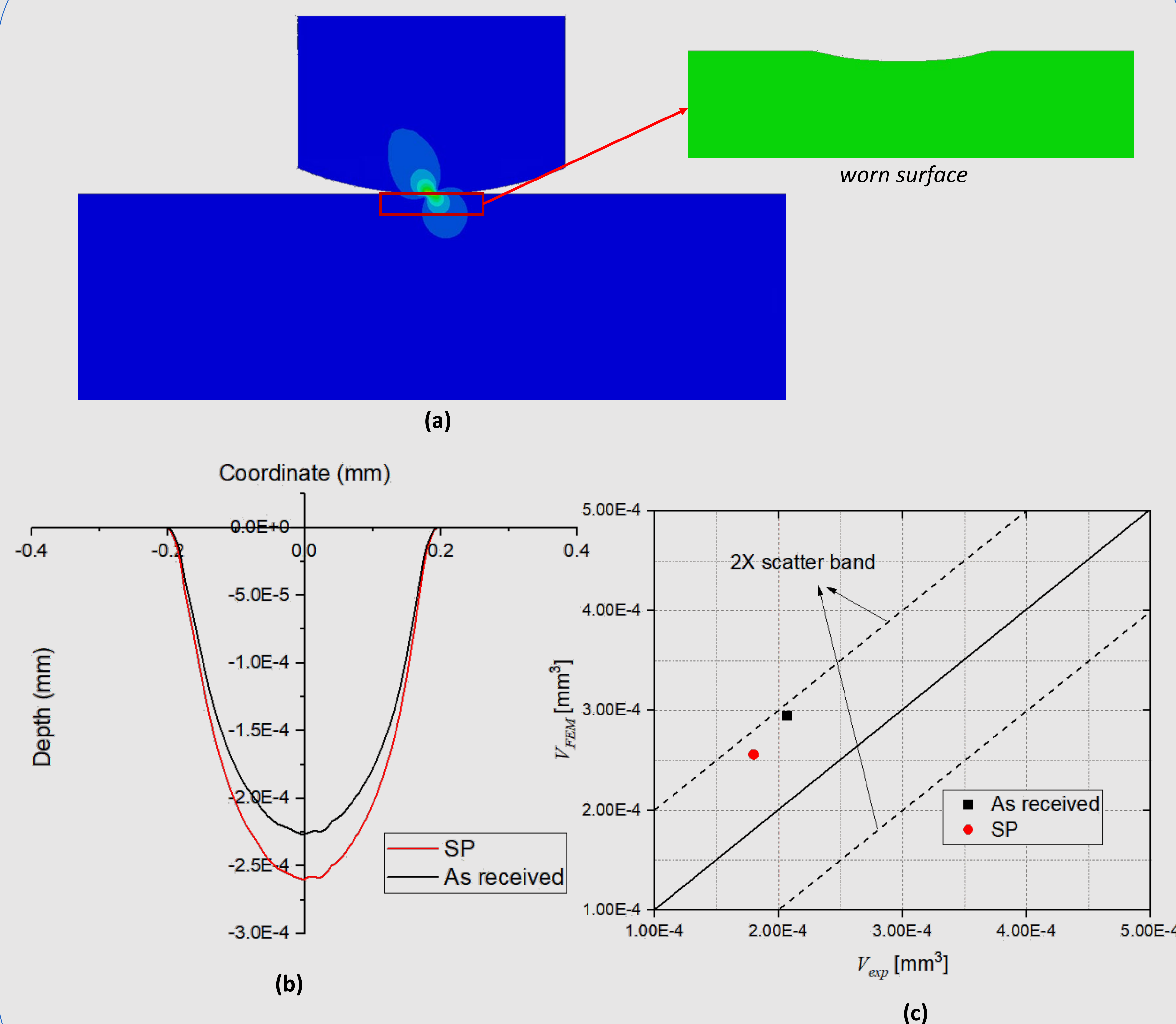
Fig. 3. The process of fretting wear and worn surface in FEM (a), wear profile after 1000 cycles (b), and wear volume comparison between FEM results and experimental measurements (c).
